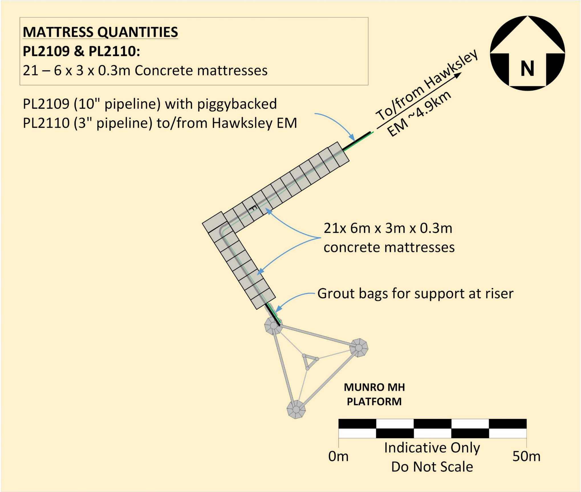
Figure A1.6.1: Schematic of pipelines near Munro MH
