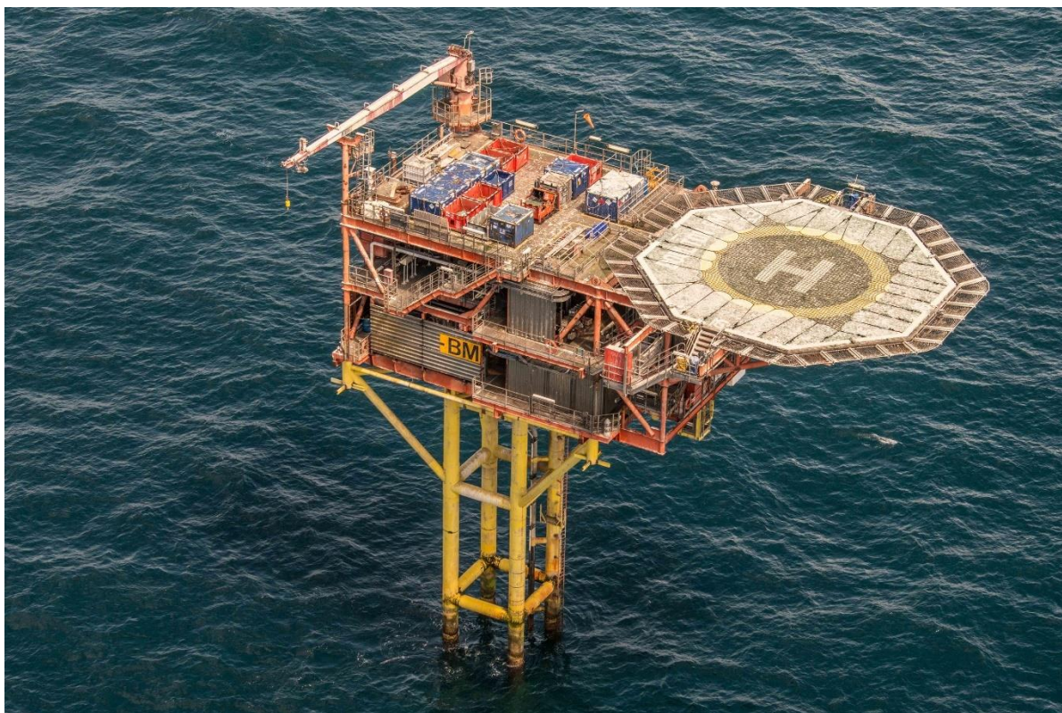
Figure 2.1.1: Photograph of the Boulton BM installation
