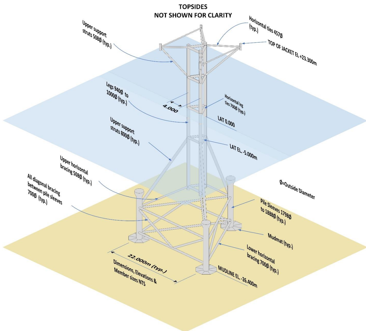
Figure 3.2.2: Katy KT Jacket 3D View
